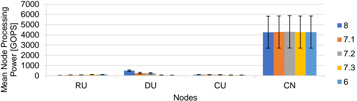
Figure J.2. Mean processing power on the network nodes in different splitting options RU-DU-CU architecture on DL.
