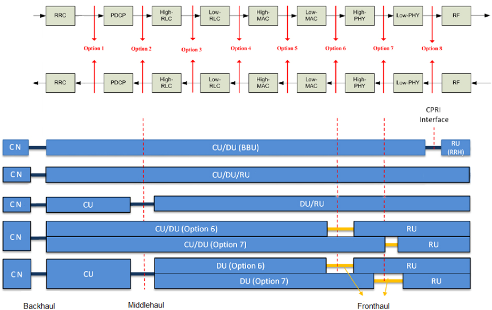
Figure 3.2. Mapping of CU, DU and RU function according to the split points (adapted from [ITUT18]).
