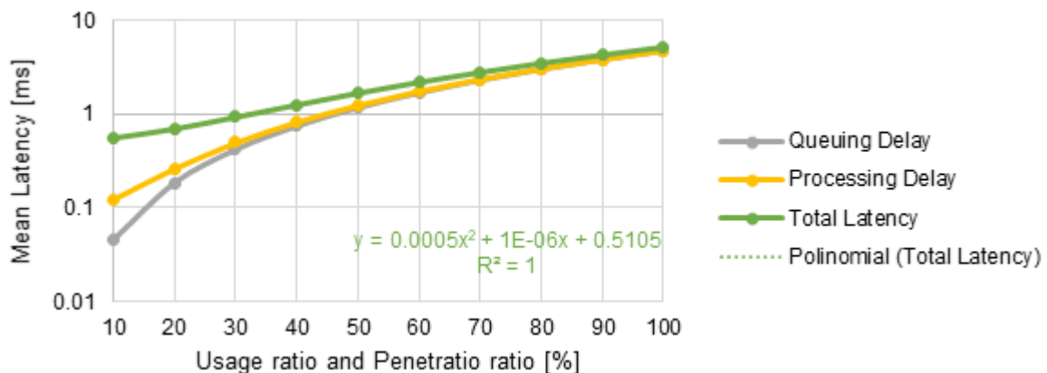
Figure 4.15. Mean network latency with variable usage and penetration ratio.
