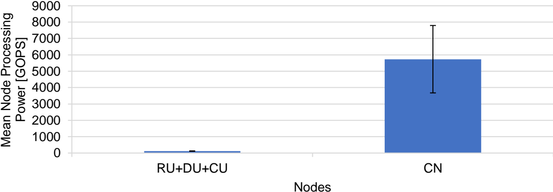
Figure J.3. Mean processing power on the network nodes for RU+DU-CU architecture on DL.
