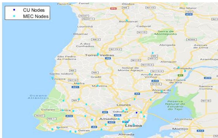
Figure N.8. CU and MEC node state for a maximum 0.25 ms E2E maximum latency in Lisbon.
