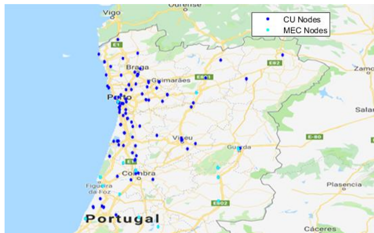
Figure M.2. CU and MEC node state for a maximum 10 ms E2E maximum latency in the north of Portugal.
