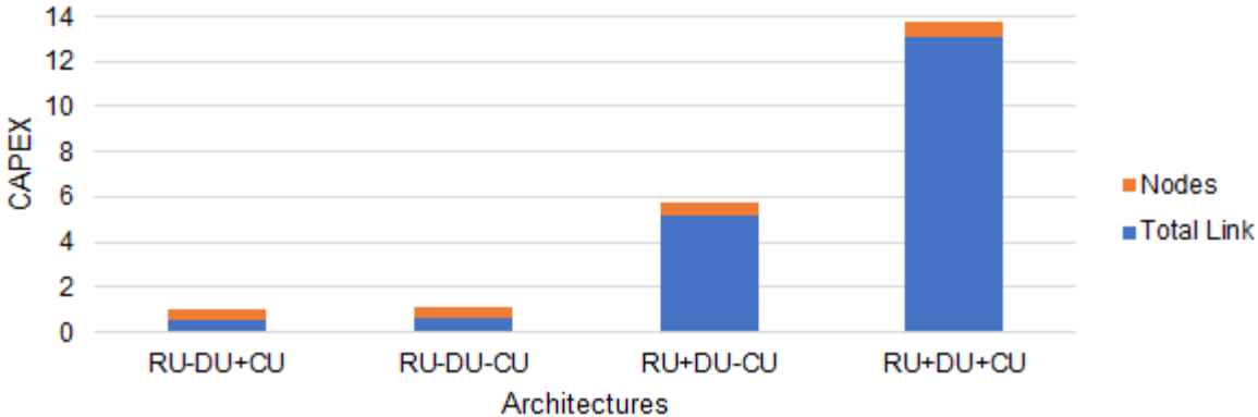
Figure 4.24. CAPEX comparison between all architectures.
