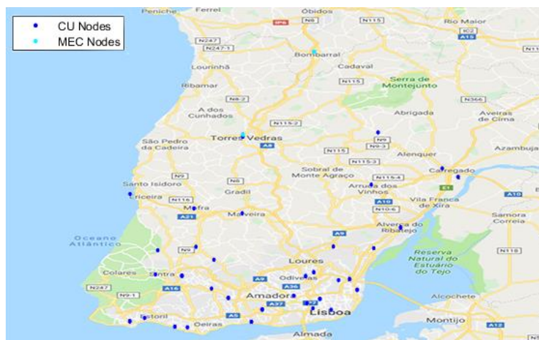
Figure N.2. CU and MEC node state for a maximum 10 ms E2E maximum latency in Lisbon.
