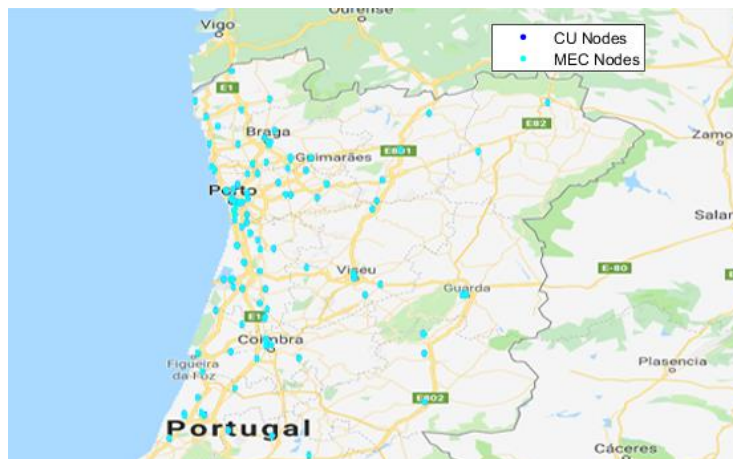
Figure M.8. CU and MEC node state for a maximum of 0.25 ms E2E maximum latency in the north of Portugal.
