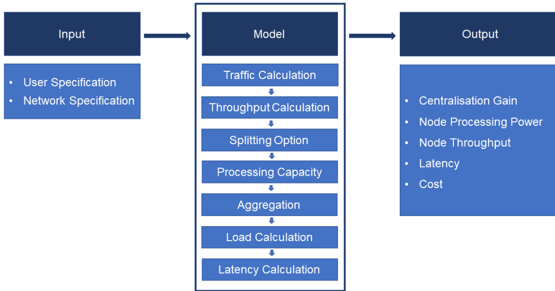
Figure 3.1. Model overview
