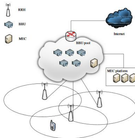
Figure 2.6. C-RAN and MEC system combination architecture (adapted from [LiHW18]).
