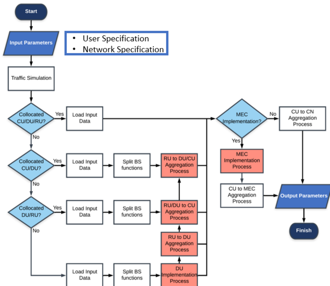
Figure 3.5. Model Flowchart
