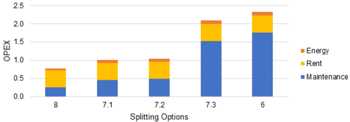
Figure 4.21. OPEX for RU-DU+CU architecture with different splitting options.
