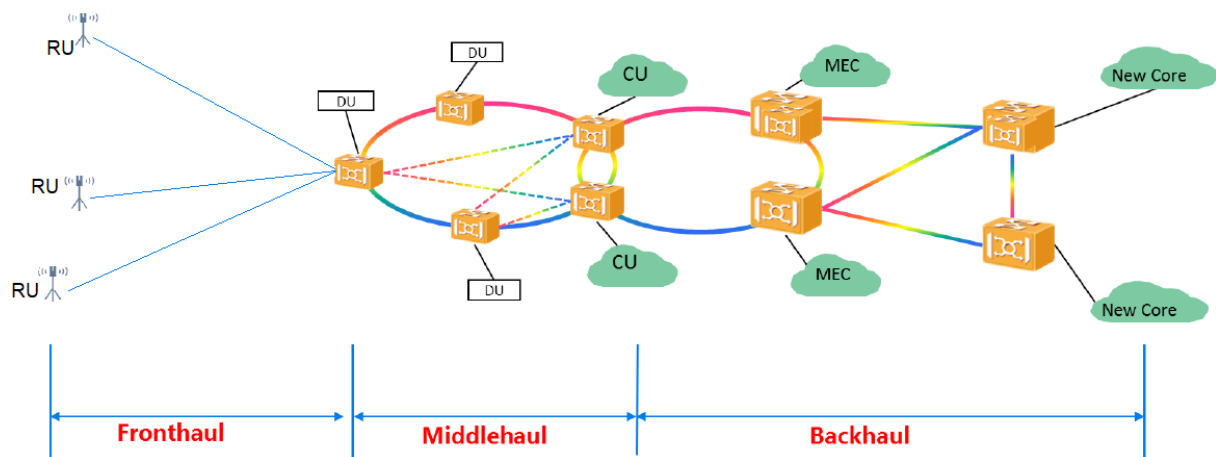
Figure 3.3. General network architecture (adapted from [ITUT18]).
