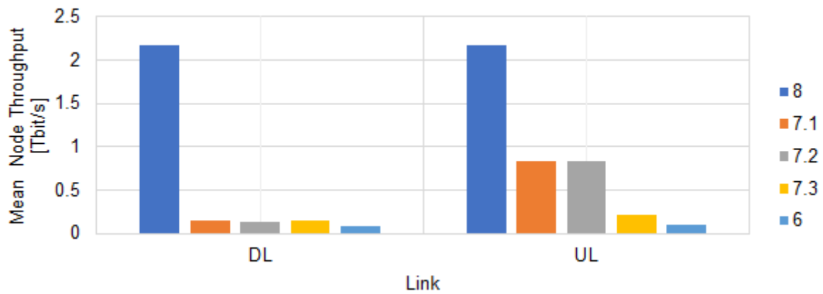
Figure F.3. Evolution of the throughput on the FH with the splitting options on the DL and UL.
